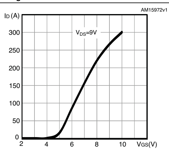
Figure 7. Transfer characteristics
