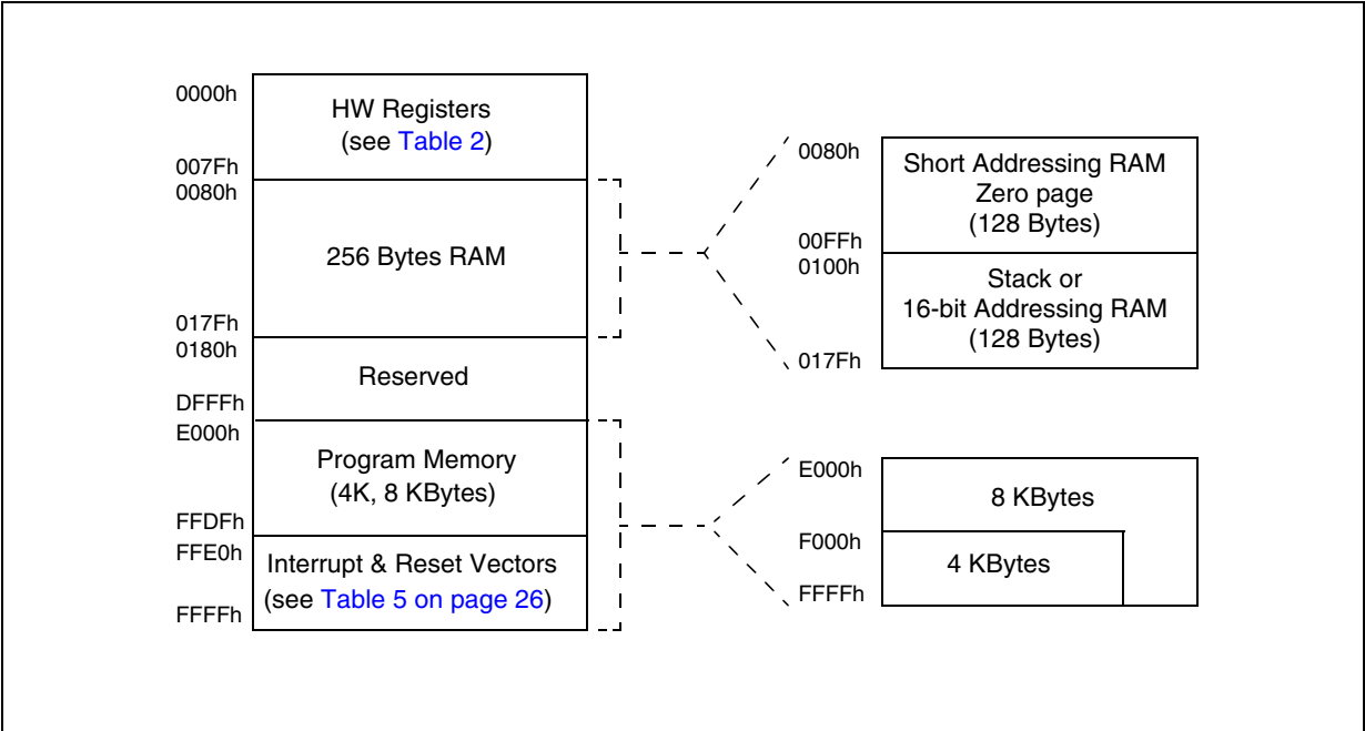
Figure 4. Memory Map
