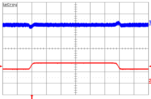
Figure 8. Output voltage response to load current step-change (12.5A–18.75A–12.5A) at V_{in}=48\text{V} . Top trace: output voltage (100mV/div.). Bottom trace: load current (10A/div.). Current slew rate: 0.1\text{ A}/\mu\text{s} . C_o = 1\mu\text{F cer} + 10\mu\text{F tant} . Time scale: 0.2ms/div.
