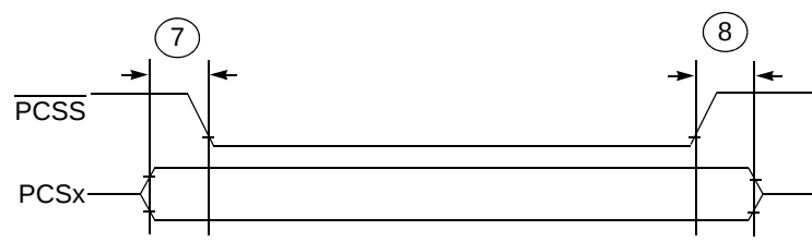
Figure 38. DSPI PCS strobe ( \overline{\text{PCSS}} ) timing
