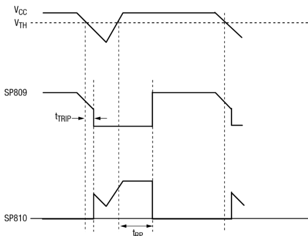
Fig. 10: Timing Waveforms
