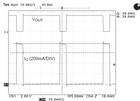
Fig. 4: Current Limit
