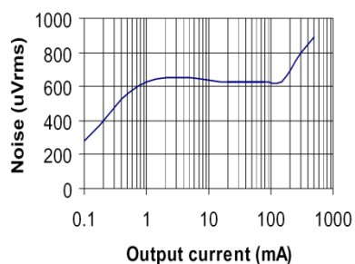
Fig. 20: Output Noise, C_{BYP} = open
