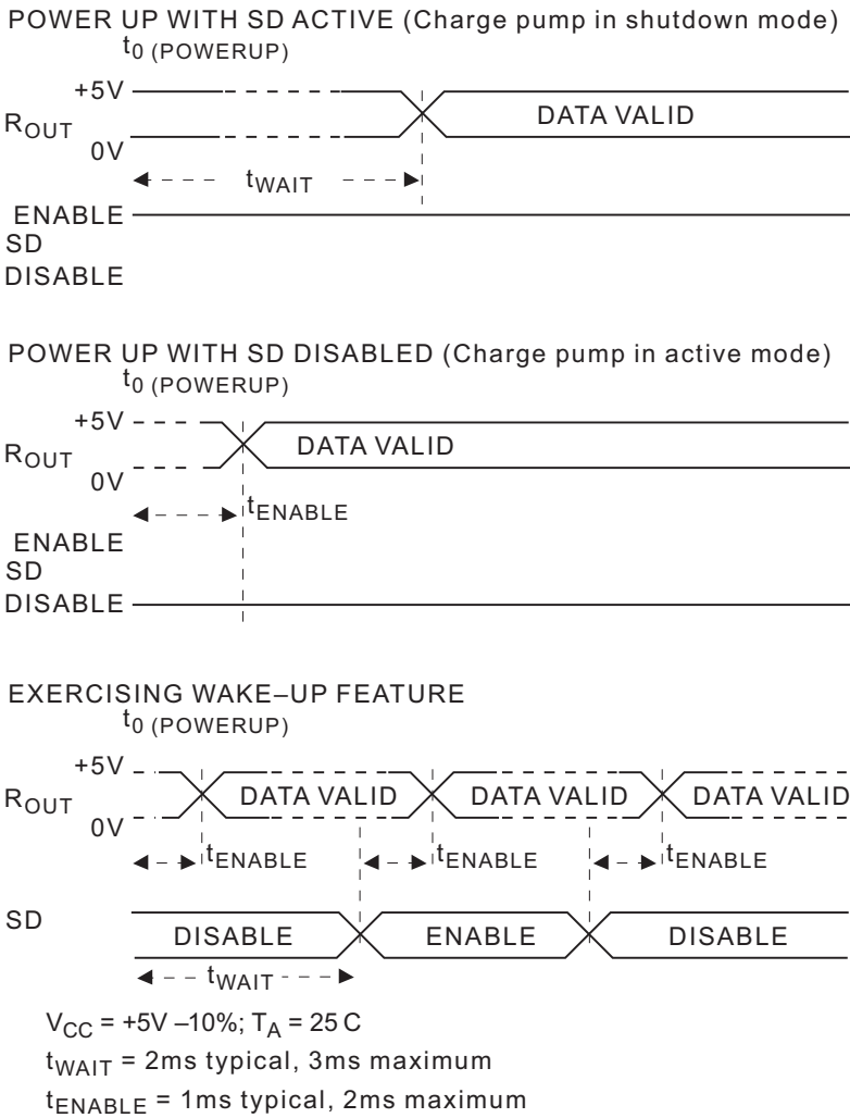
Figure 11: Wake-Up Timing
