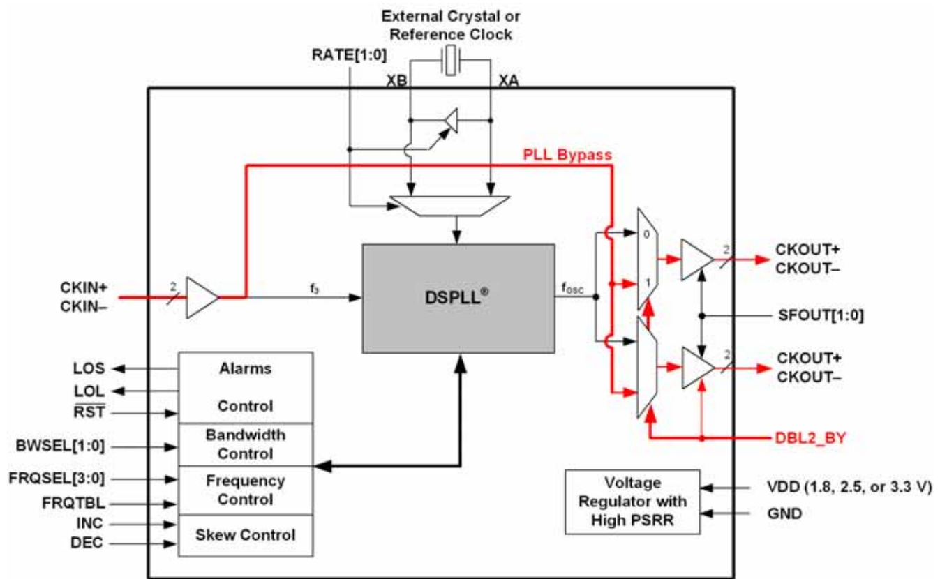
Figure 6. Bypass Signal
