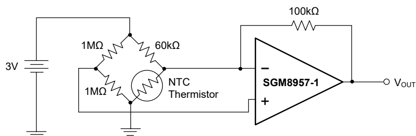
Figure 5. Thermistor Measurement
