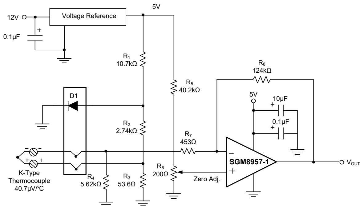
Figure 1. Temperature Measurement
