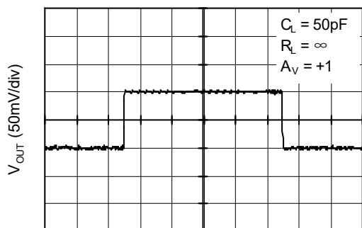
Small Signal Transient Response at +5V
