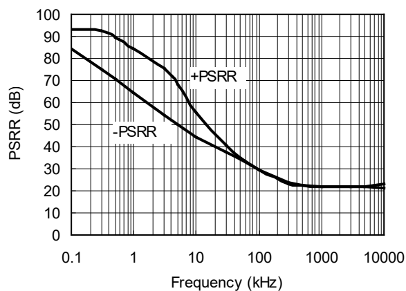
PSRR vs. Frequency at \pm 2.5\text{V}
