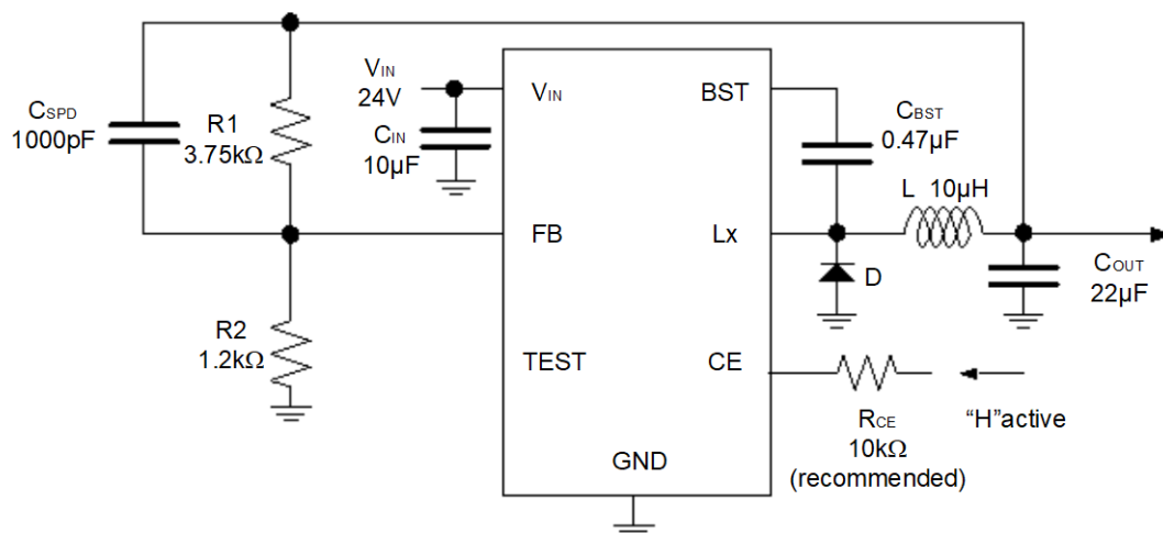
R1245x00xC/D Typical Application Circuit, 500 kHz, V_{OUT} = 3.3 V, V_{IN} = 24 V
