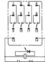
MY4N-CR
