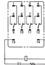
MY4-CR
