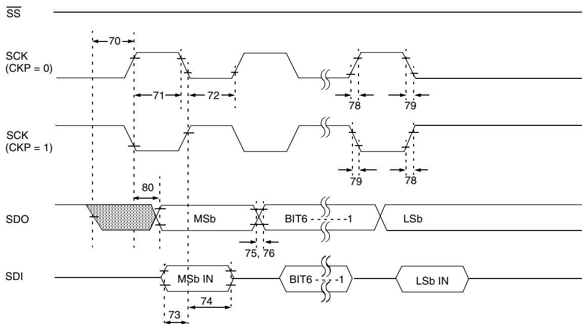
FIGURE 14-10: SPI MASTER MODE TIMING (CKE = 0, SMP = 0)
