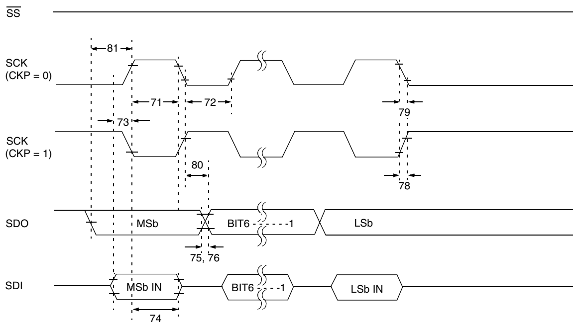
FIGURE 14-11: SPI MASTER MODE TIMING (CKE = 1, SMP = 1)
