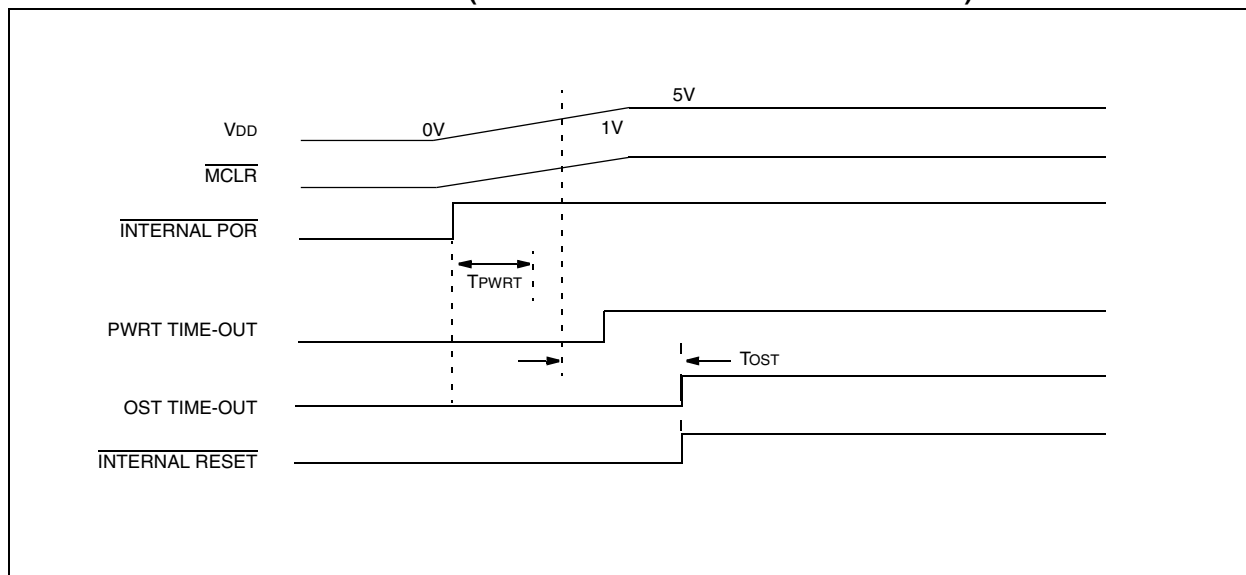
FIGURE 11-8: SLOW RISETIME ( \overline{\text{MCLR}} TIED TO V_{DD} VIA RC NETWORK)
