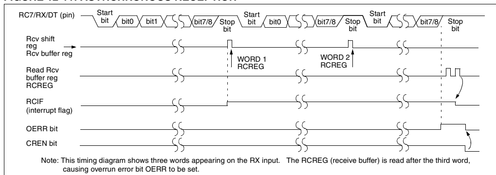
FIGURE 12-11: ASYNCHRONOUS RECEPTION
