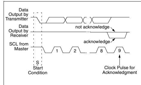
FIGURE 11-17: SLAVE-RECEIVER ACKNOWLEDGE
