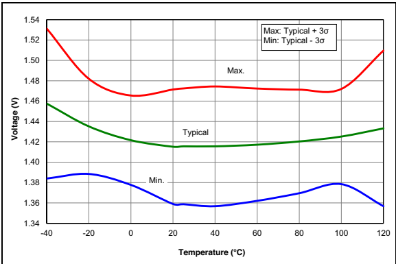
FIGURE 22-16: POR Rearm Voltage, PIC12FXXX Only
