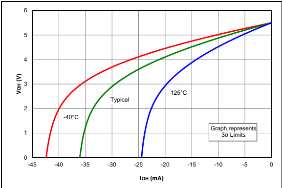
FIGURE 22-14: V_{OH} vs. I_{OH} , Over Temperature, V_{DD} = 5.5\text{V} , PIC12FXXX Only
