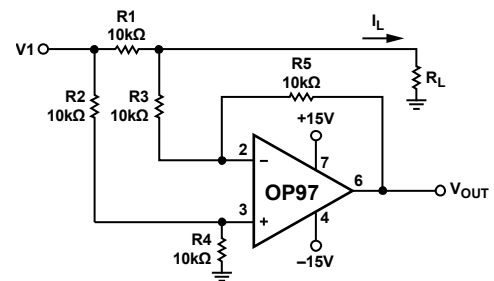
Figure 36. Current Monitor
