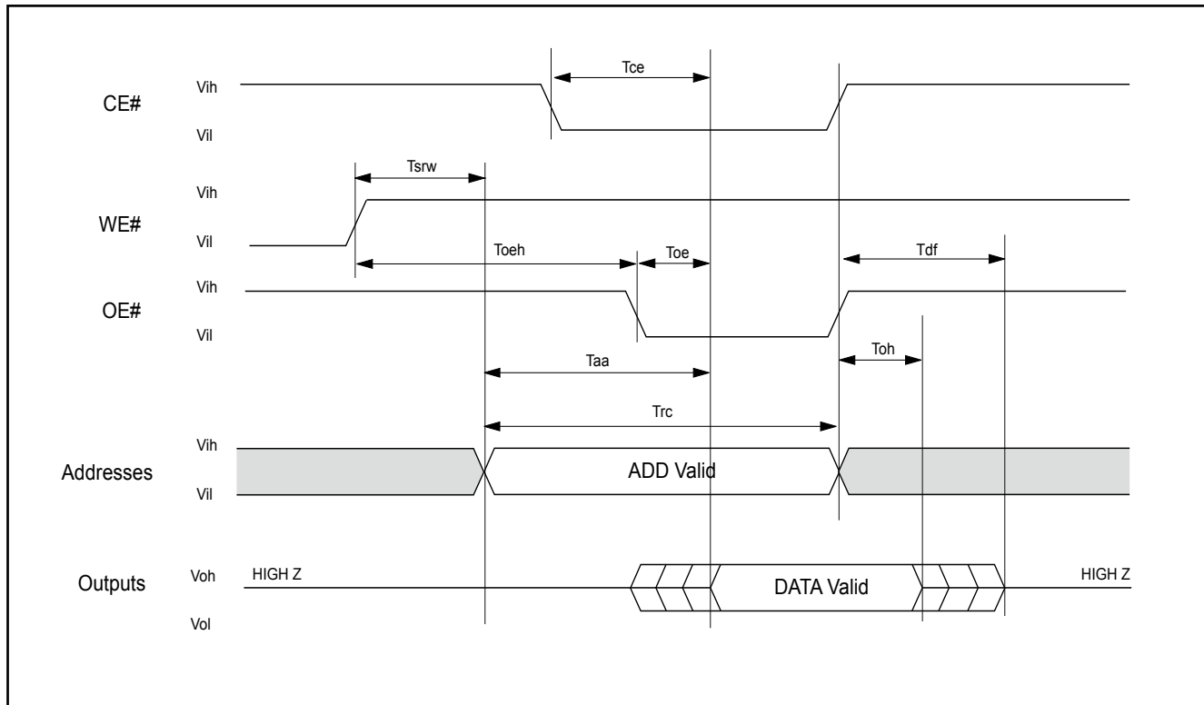
Figure 5. READ TIMING WAVEFORMS
