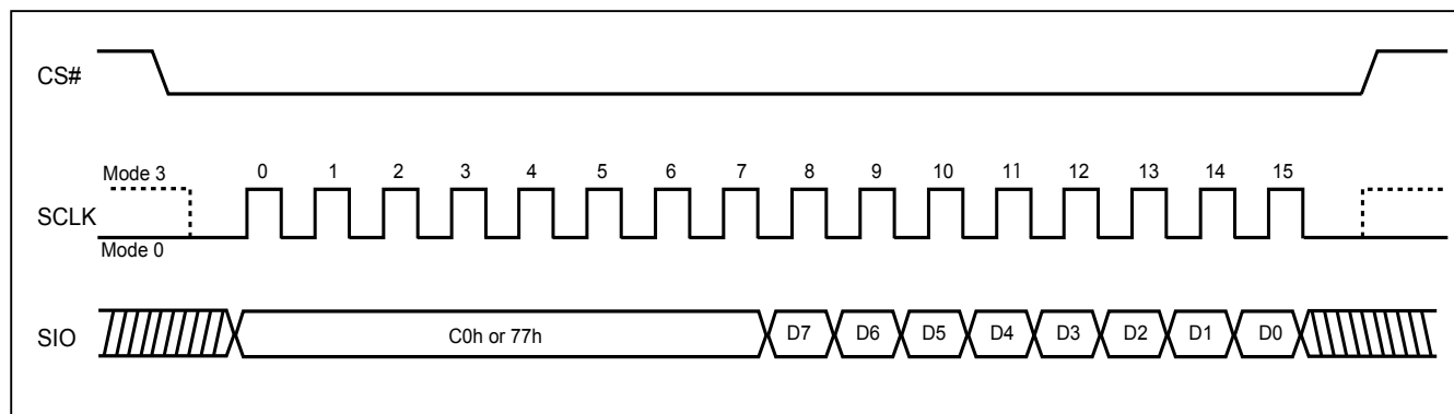
Figure 17. Burst Read
