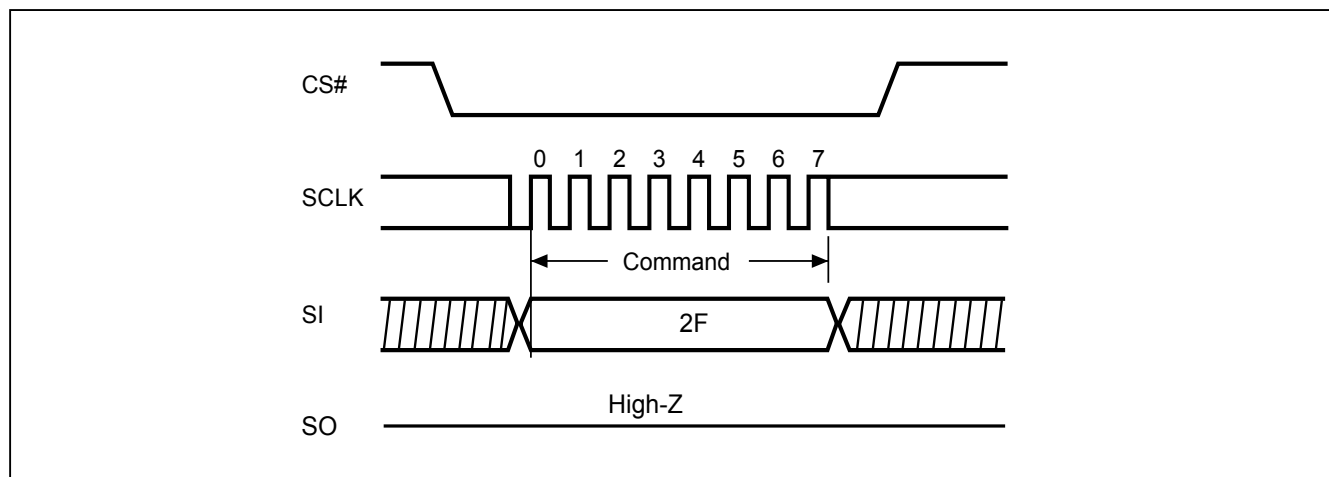
Figure 31. Write Security Register (WRSCUR) Sequence (Command 2F) (SPI mode)
