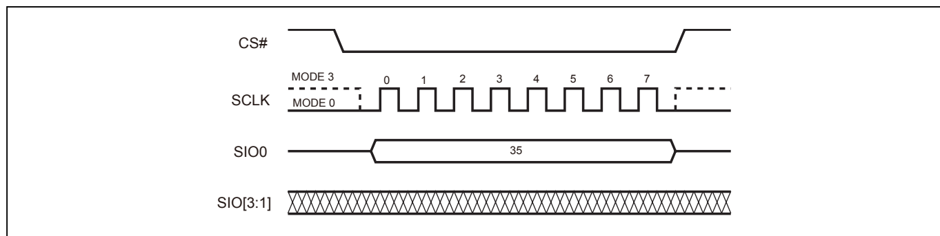
Figure 4. Enable QPI Sequence (Command 35H)
