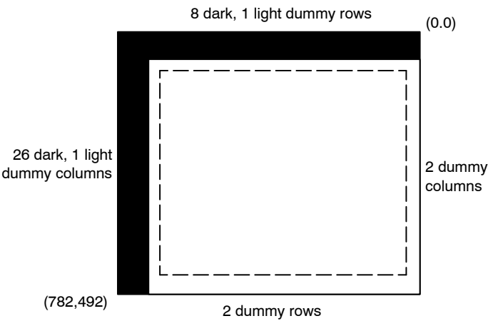
Figure 4. Pixel Array Description
