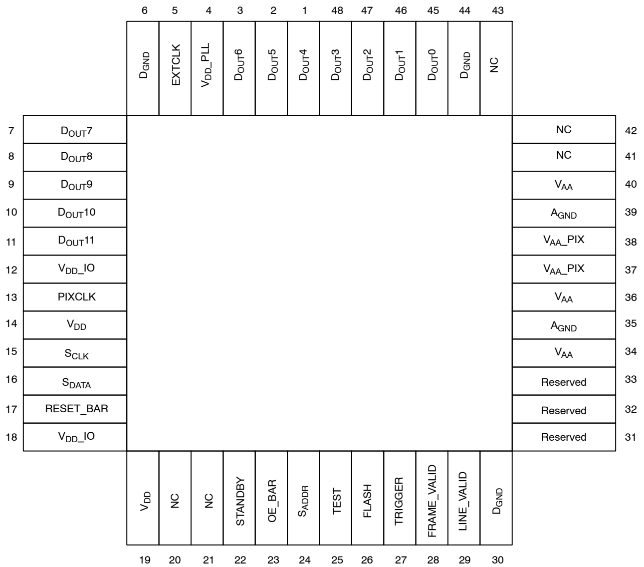
Figure 3. 48 iLCC Package, Parallel Output
