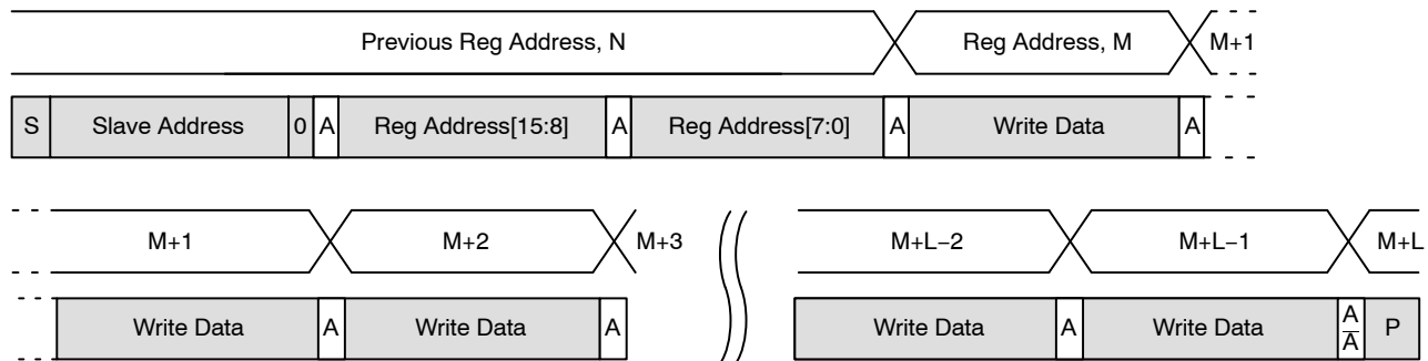
Figure 23. Sequential WRITE, Start at Random Location
