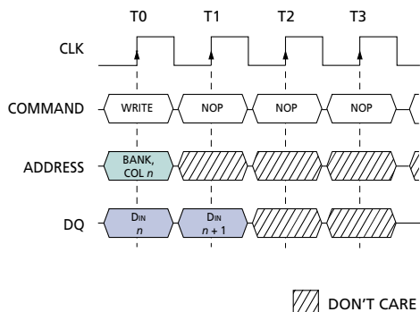
Figure 17: WRITE Burst
