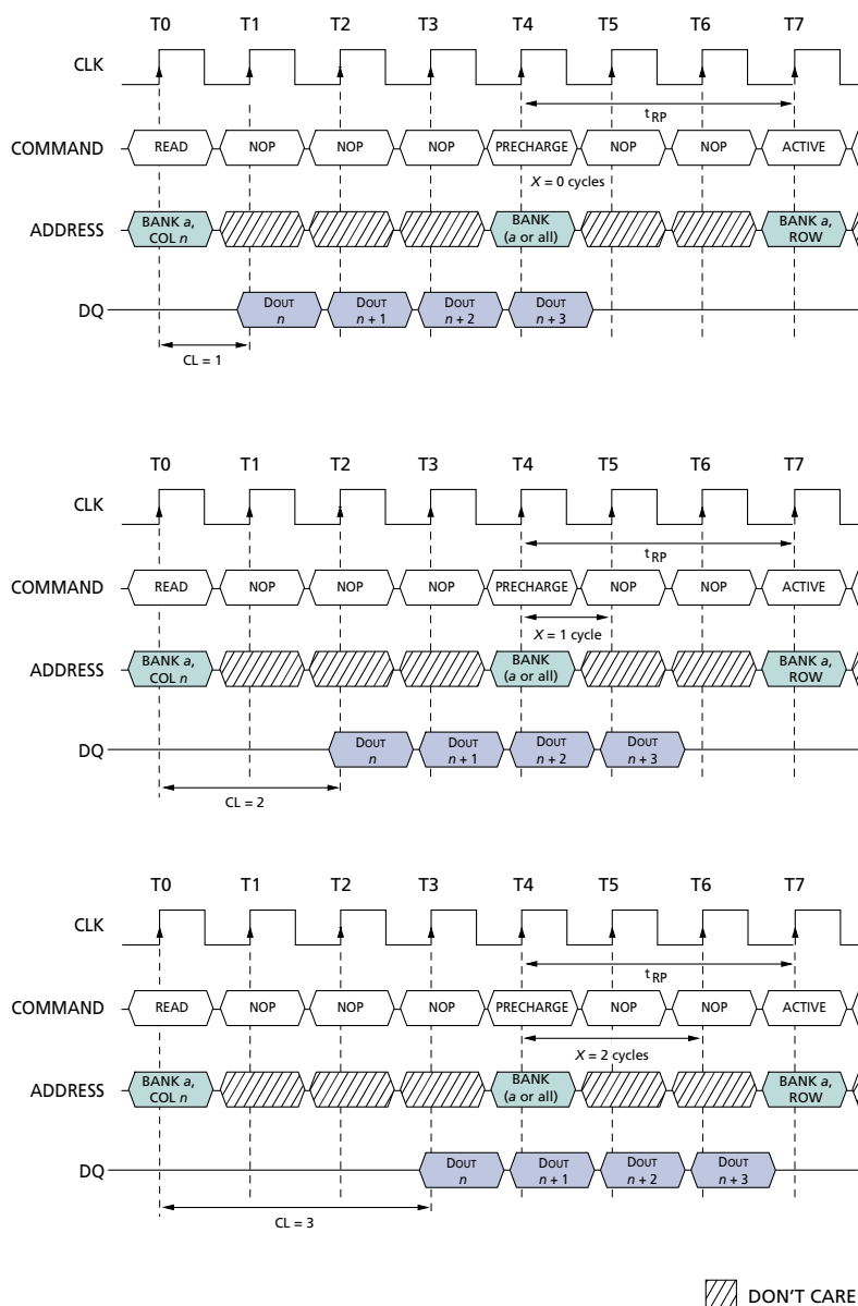
Figure 14: READ-to-PRECHARGE
