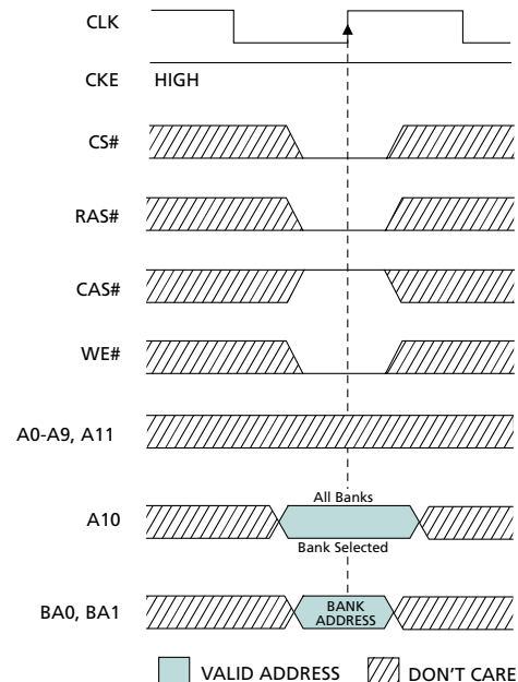
Figure 23: PRECHARGE Command
