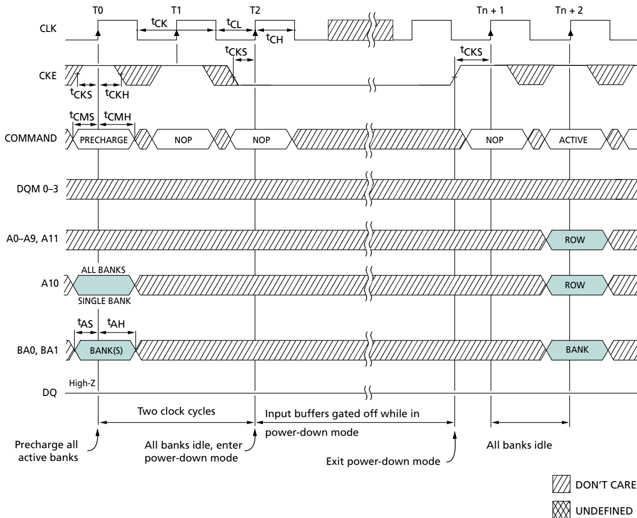
Figure 32: Power-Down Mode
