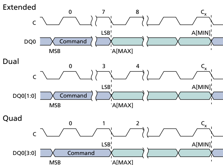
Figure 39: SUBSECTOR and SECTOR ERASE Timing
