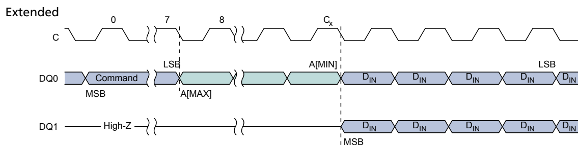
Figure 35: DUAL INPUT FAST PROGRAM Command
