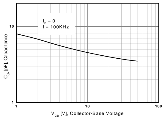
Figure 5. Collector-Base Capacitance
