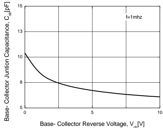
Figure 6. Collector-Base Capacitance
