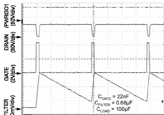
Auto-Retry Response
