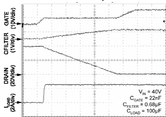
Turn-On Response
