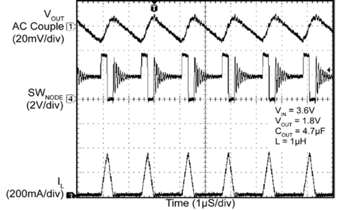
Switching Waveform Discontinuous Mode (50mA)
