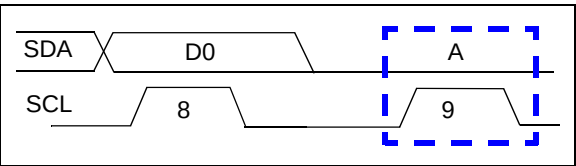
FIGURE 6-4: Acknowledge Waveform.
