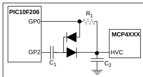
FIGURE 8-2: MCP4XXX Nonvolatile Digital Potentiometer Evaluation Board (MCP402XEVB) Implementation to Generate the V_{IH} Voltage.
