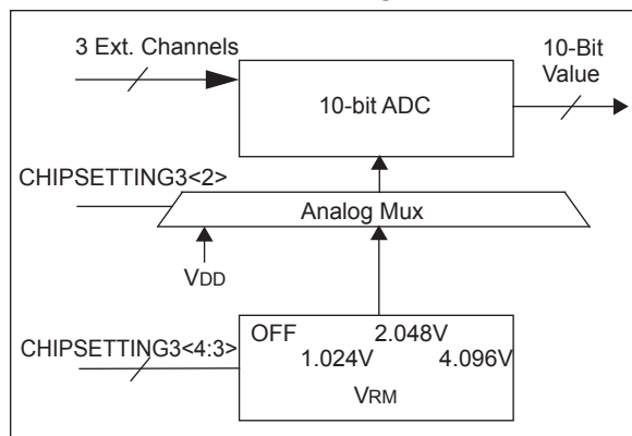
FIGURE 1-6: ADC SUB-MODULE DETAILS
