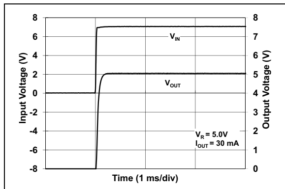
FIGURE 2-37: Start-up Response.
