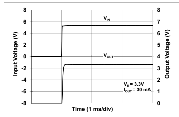
FIGURE 2-35: Start-up Response.
