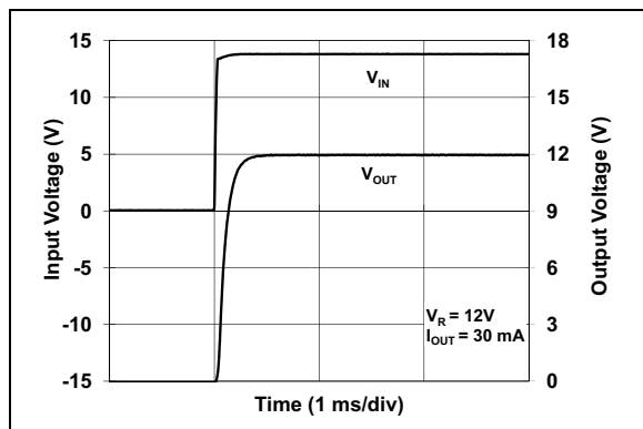
FIGURE 2-39: Start-up Response.
