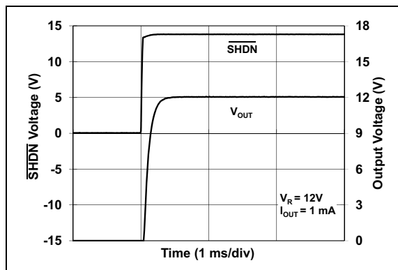
FIGURE 2-42: SHDN Response.
