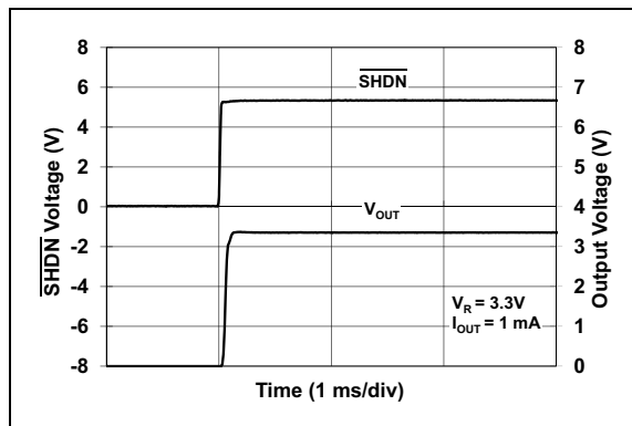
FIGURE 2-40: SHDN Response.
