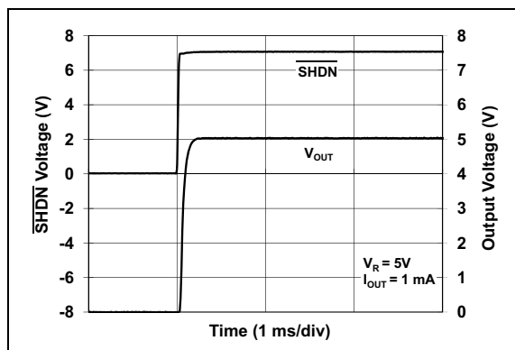
FIGURE 2-41: SHDN Response.
