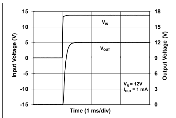
FIGURE 2-38: Start-up Response.
