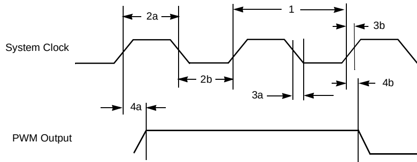
Figure 70. PWM Timing
