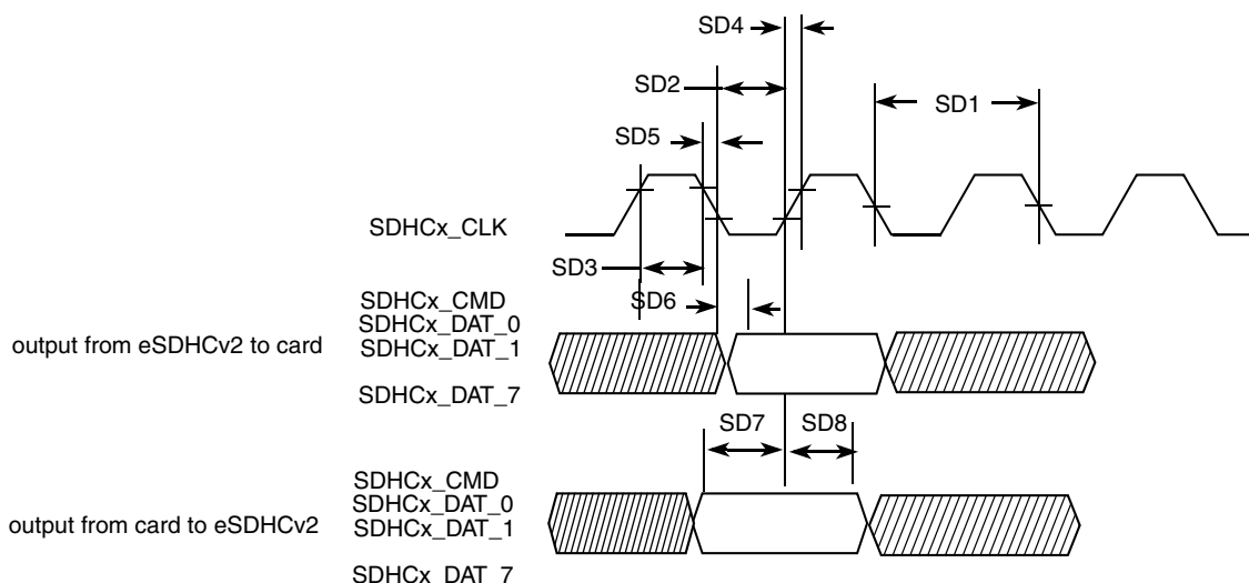
Figure 38. eSDHCv2 Timing
