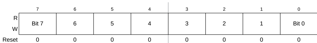
Figure 16-14. TPM Channel Value Register Low (TPMxCnVL)
