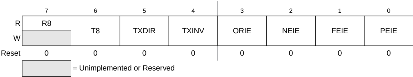
Figure 14-10. SCiX3 Control Register 3 (SCiX3)
