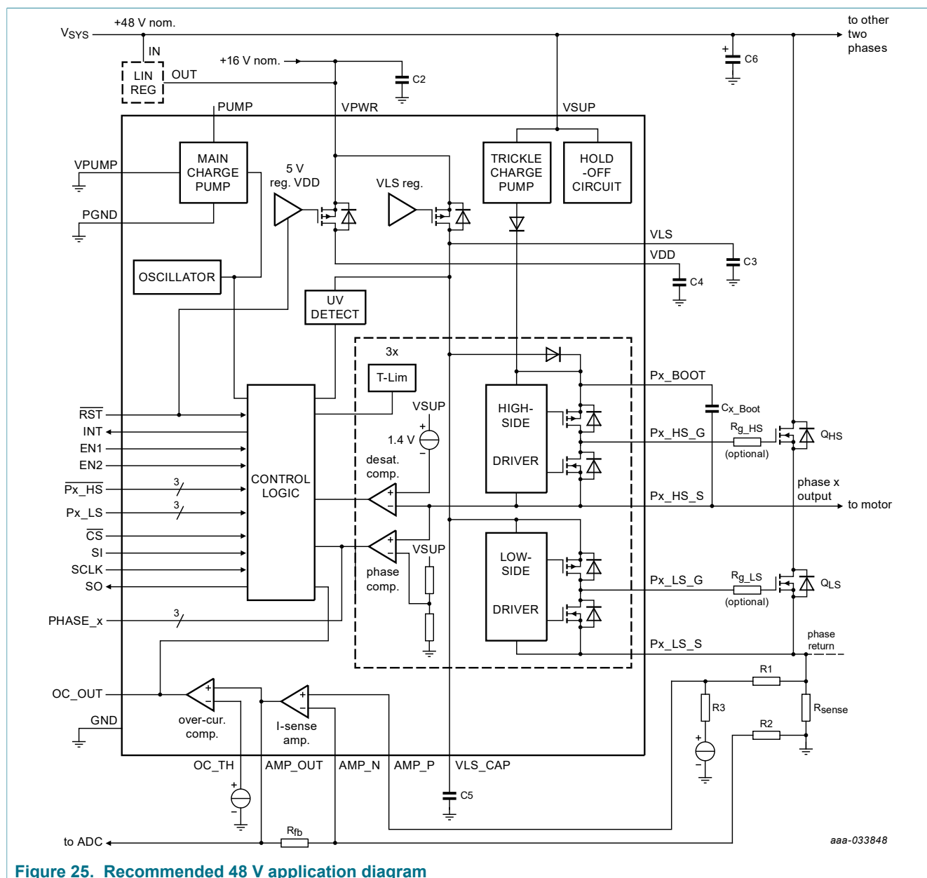
Figure 25. Recommended 48 V application diagram
