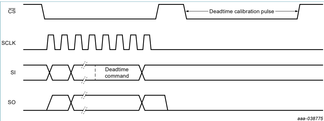
Figure 18. Deadtime calibration
