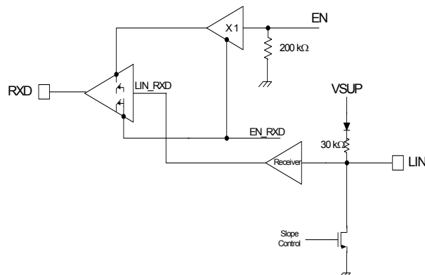
Figure 28. RXD Interface
