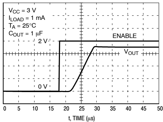
Figure 21. Enable Response
