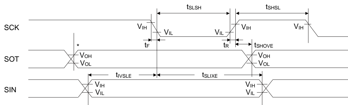
Slave mode
