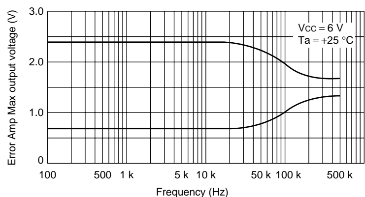
Error Amp Max output voltage vs. Frequency
