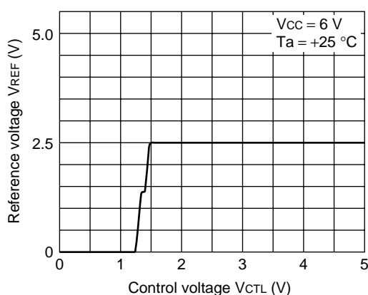
Reference voltage vs. Control voltage
