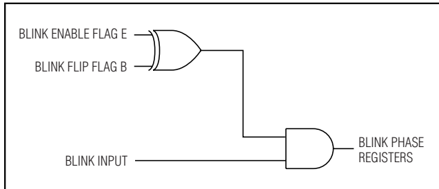
Figure 11. BLINK Logic
