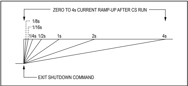
Figure 4. Ramp-Up Behavior
