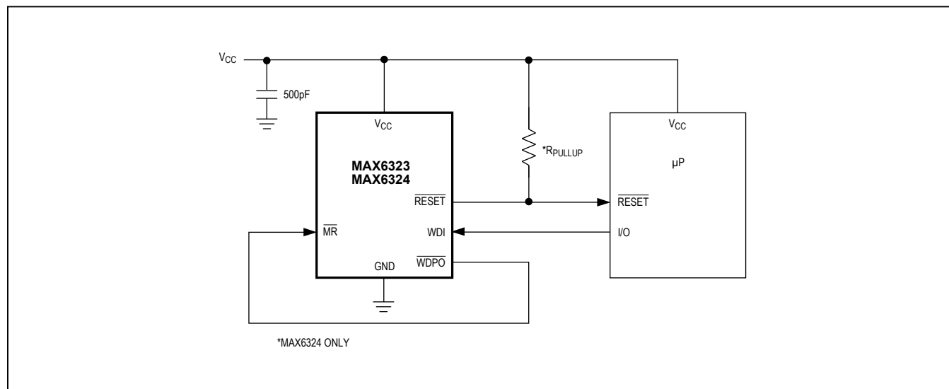
Figure 10. WDPO to MR Loopback Circuit
