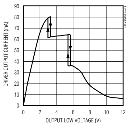
DRIVER OUTPUT CURRENT vs. OUTPUT LOW VOLTAGE
