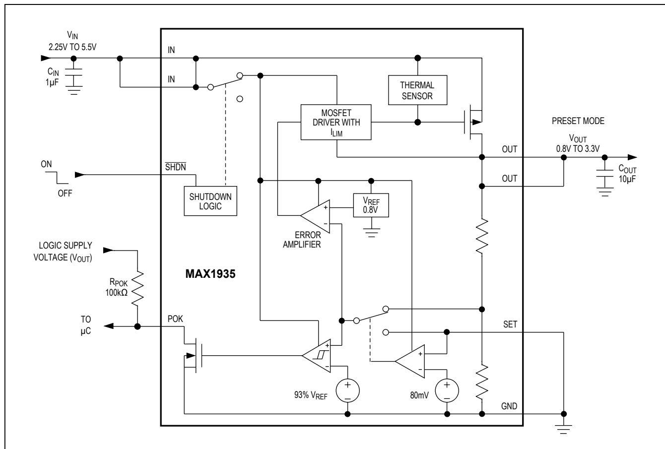
Figure 1. Functional Diagram
