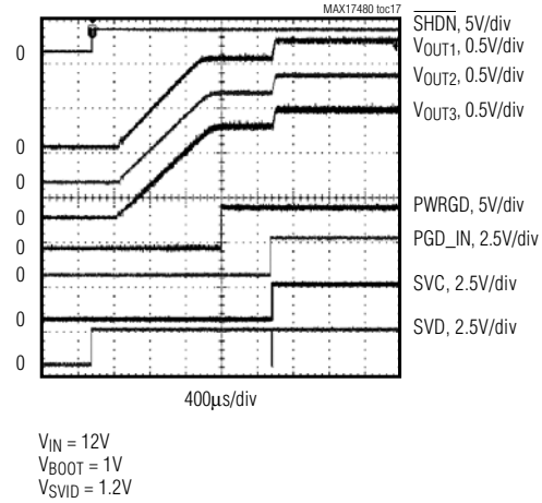
STARTUP SEQUENCE
