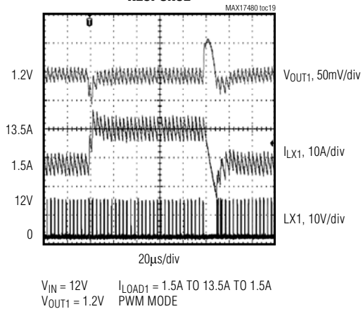
CORE SMPS 1-PHASE LOAD-TRANSIENT RESPONSE
