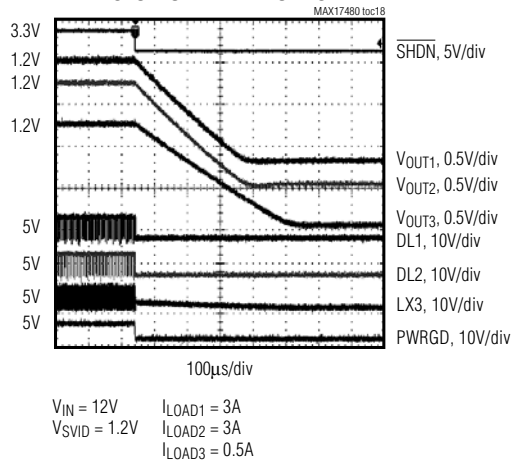
SHUTDOWN WAVEFORMS
