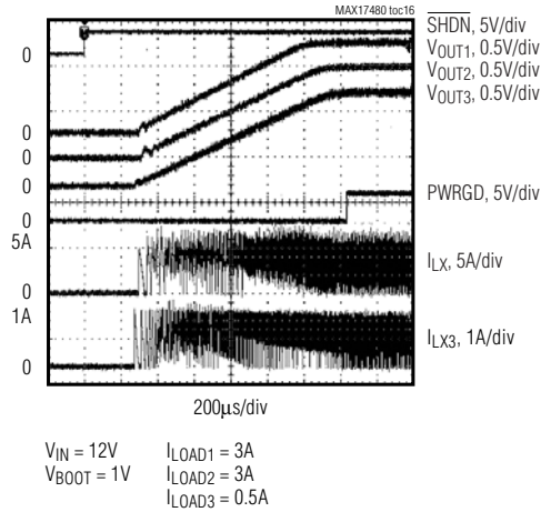
STARTUP WAVEFORMS
