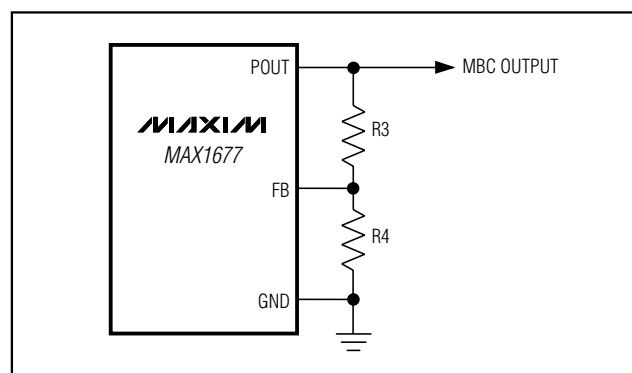
Figure 8. Setting the MBC Output Voltage Externally
