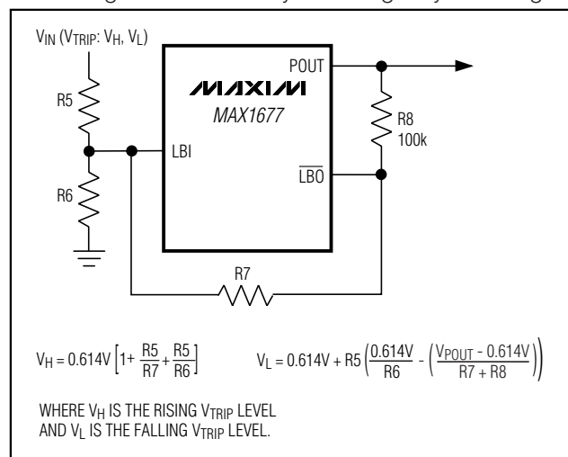
Figure 7. Adding External Hysteresis to the LBI Comparator
