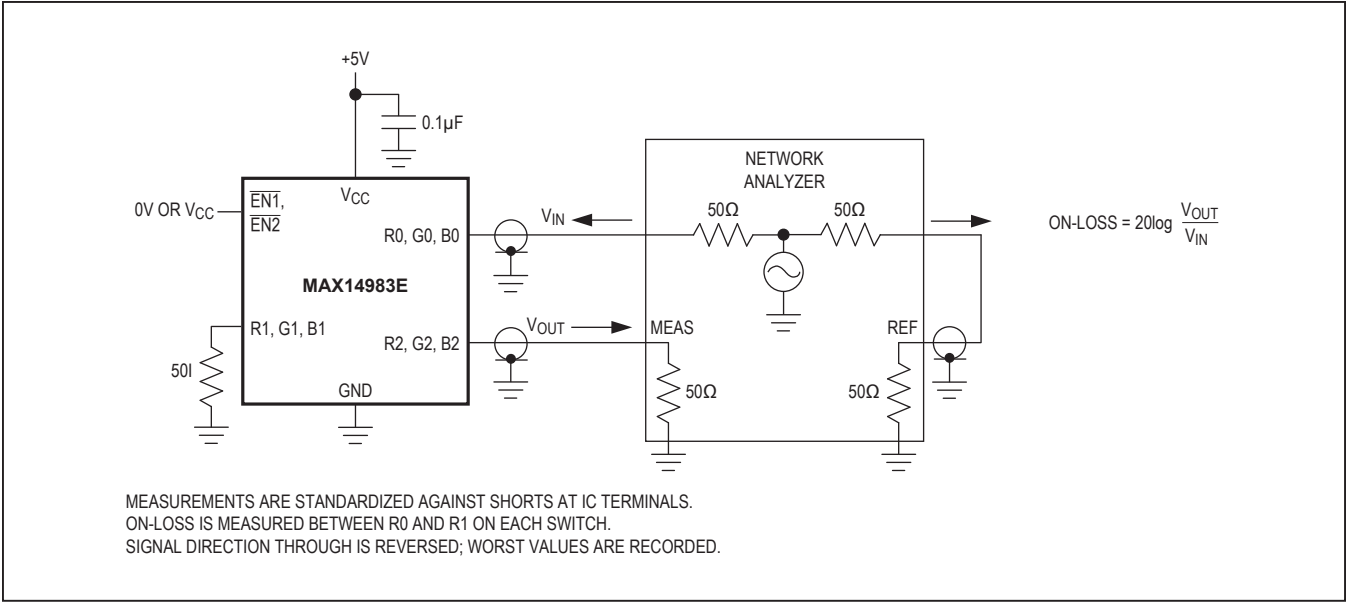
Figure 1. On-Loss
