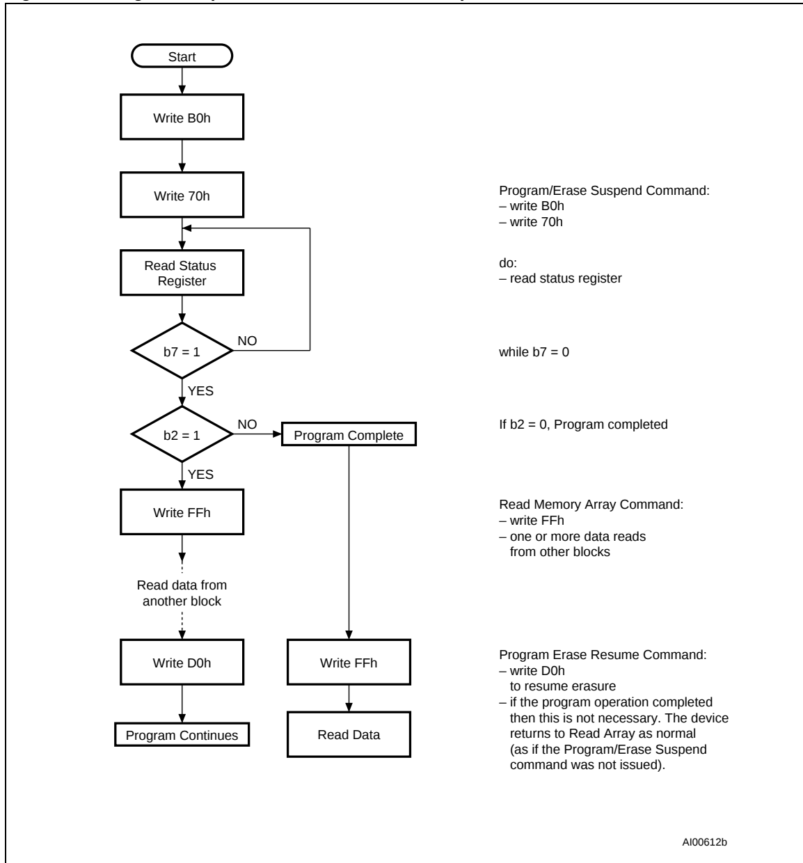
Figure 23. Program suspend &amp; resume flowchart and pseudocode
