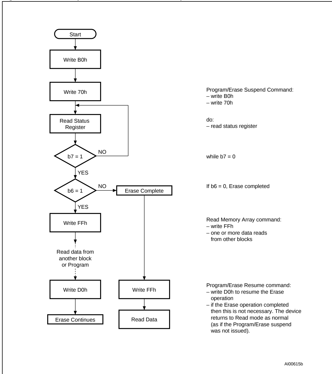
Figure 25. Erase suspend &amp; resume flowchart and pseudocode
