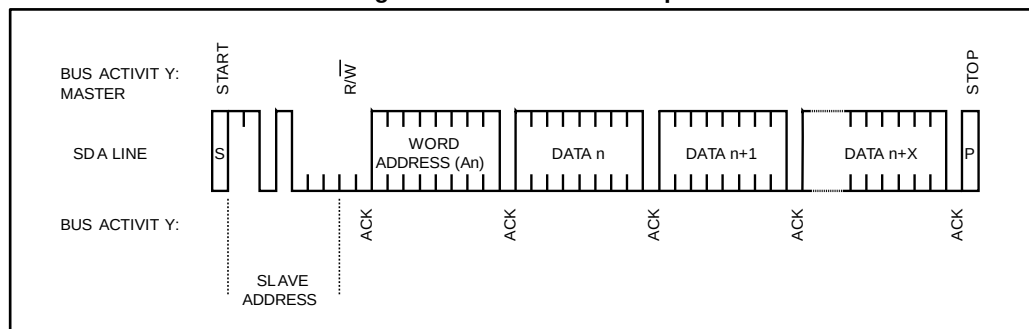
Figure 12: WRITE mode sequence
