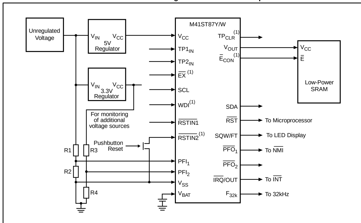
Figure 5: Hardware hookup
