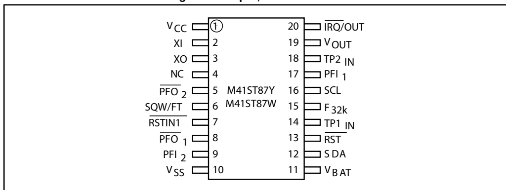
Figure 3: 20-pin, SSOP connections
