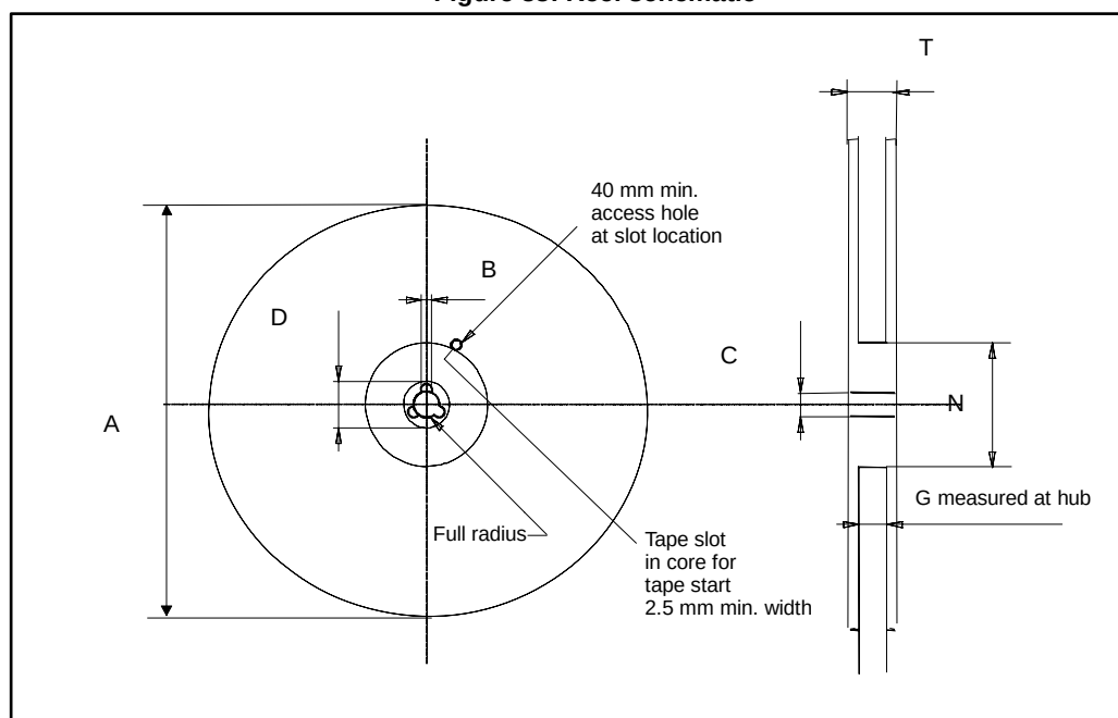
Figure 33: Reel schematic
