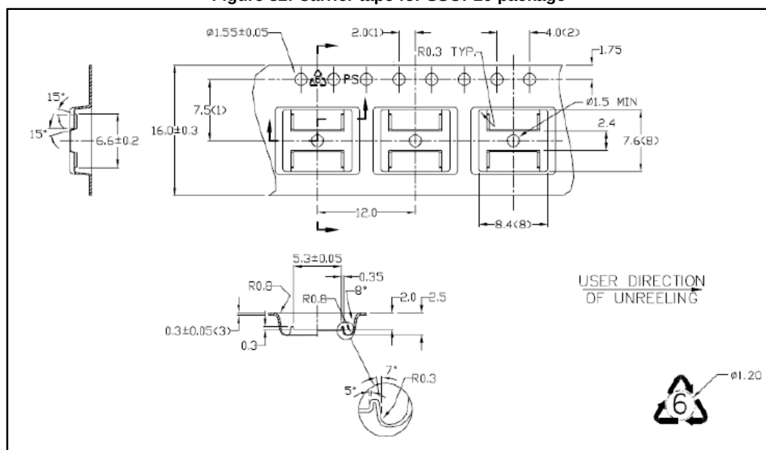
Figure 32: Carrier tape for SSOP20 package
