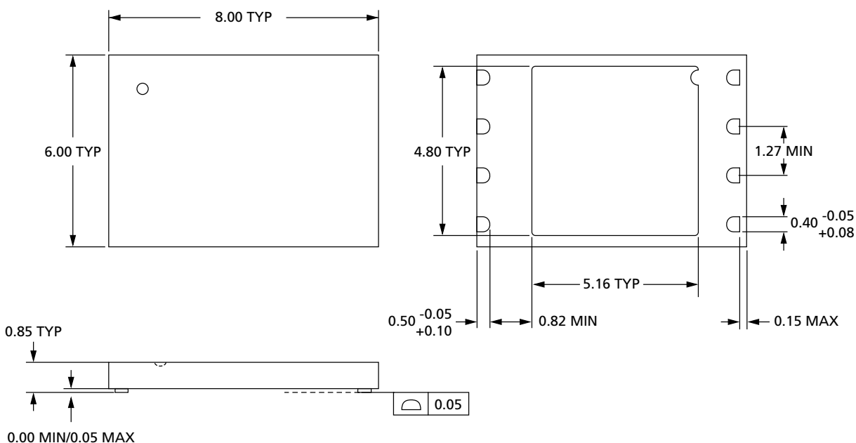
Figure 34: VFDFPN8 (MLP8) 8mm x 6mm
